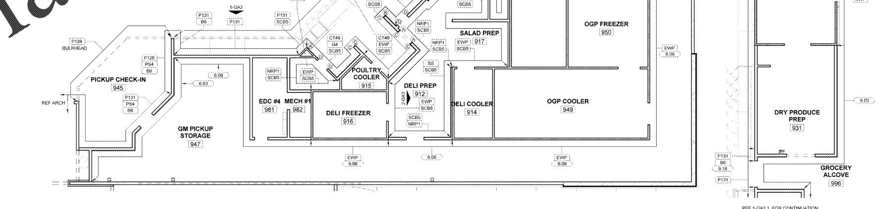
1 ENLARGED FRONT GROCERY FINISH PLAN 1/8" x 1'-0"
