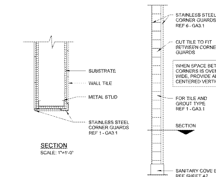
5 DETAIL AT WALL END 1/2" x 1/2"
