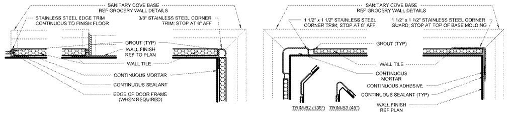
6 STAINLESS STEEL CORNER GUARD AND TRIM DETAILS 6" x 1/2"
