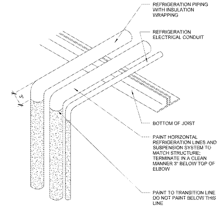
7 REFRIGERATION DROP LINES 1/2" x 1/2"
