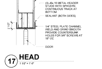
17 HEAD 1 1/2" x 1'-0"
