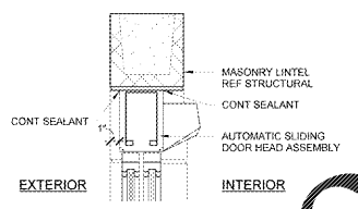
6 HEAD 1 1/2" x 1'-0"
