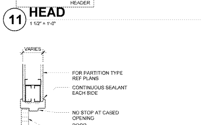
11 HEAD 1 1/2" x 1'-0"
