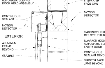
19B HEAD 1 1/2" x 1'-0"
