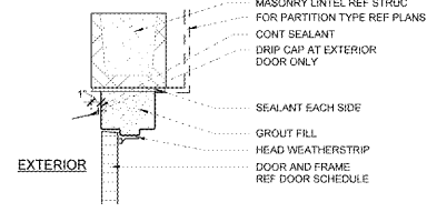
15 HEAD 1 1/2" x 1'-0"
