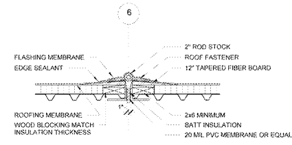
15 EXPANSION JOINT 1" x 1'-0"
