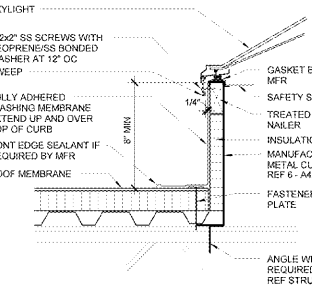
9 SKYLIGHT CURB 1 1/2" x 1'-0"
