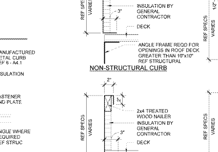
6 CURB 1 1/2" x 1'-0"
