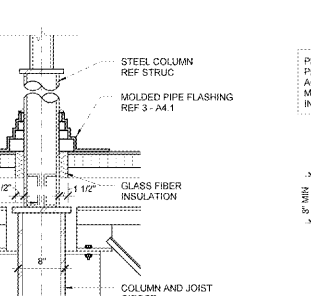
4 FLUE PENETRATION 1" x 1'-0"
