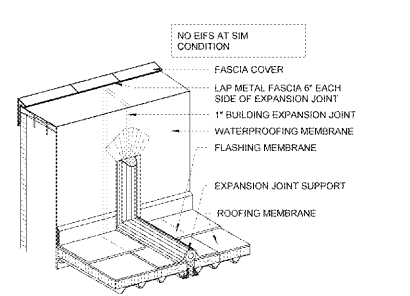
11 EXPANSION JOINT 3/4" x 1'-0"
