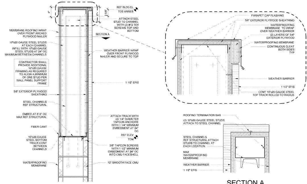
16 PARAPET COPING 1 1/2" x 1'-0"
