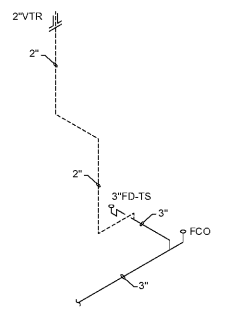
WASTE AND VENT PIPING P 1
