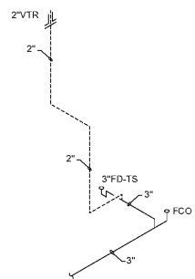
WASTE AND VENT PIPING P 1
