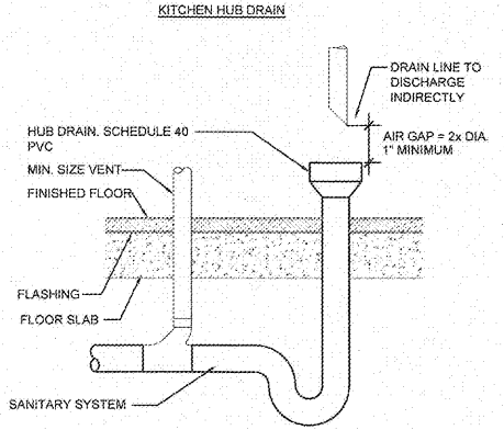
HUB DRAIN DETAIL SCALE: NONE 4
