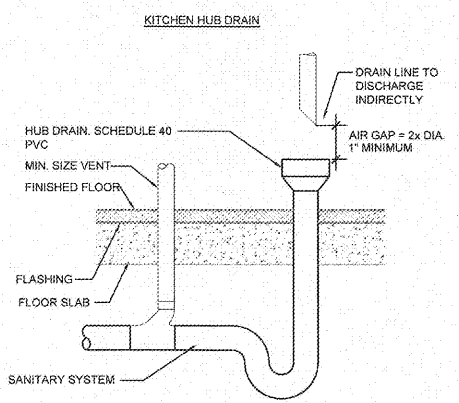
HUB DRAIN DETAIL SCALE: NONE 4
