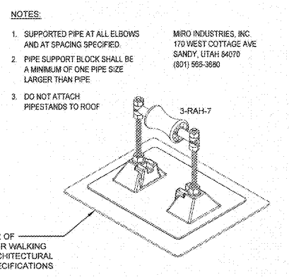
ROOF PIPING SUPPORT DETAIL (IF REQ'D) SCALE: NONE 3
