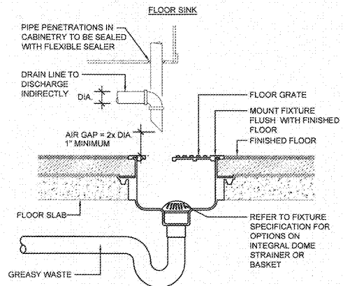
INDIRECT DRAINAGE DETAILS SCALE: NONE 1
