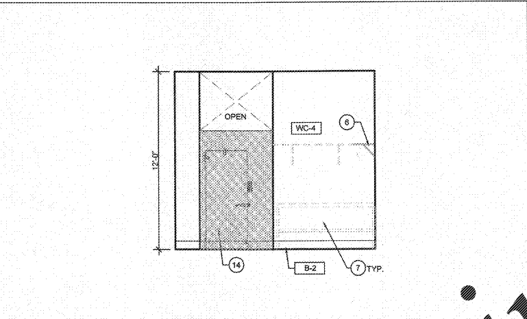
INTERIOR ELEVATION 3 1/4"=1'-0"
