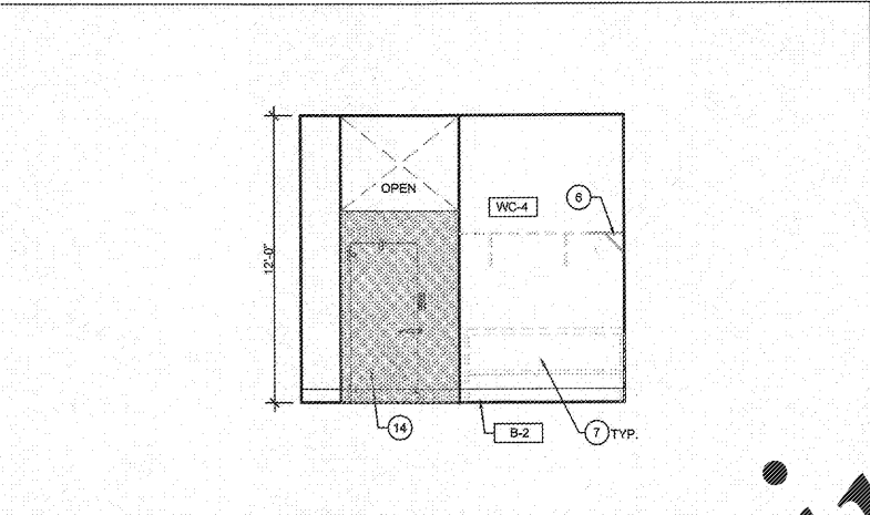
INTERIOR ELEVATION 3 1/4"=1'-0"
