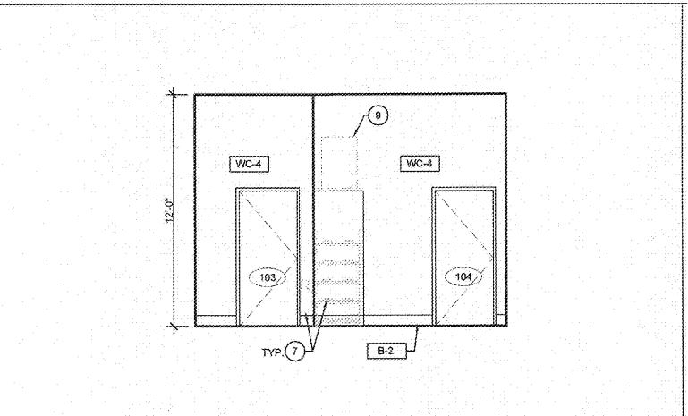
INTERIOR ELEVATION 2 1/4"=1'-0"
