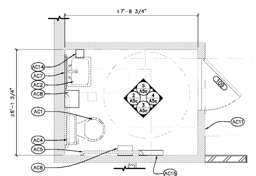
1 TOILET ROOM PLAN A5c SCALE 1/2" = 1'-0"
