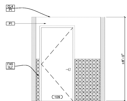
4 TOILET ROOM ELEVATION A5c SCALE 1/2" = 1'-0"
