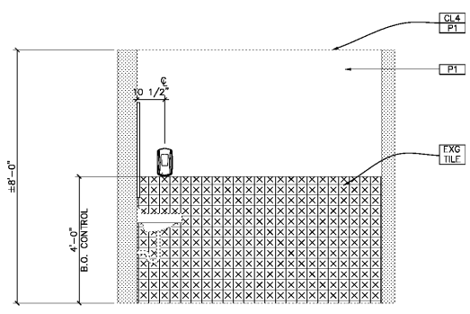
5 TOILET ROOM ELEVATION A5c SCALE 1/2" = 1'-0"
