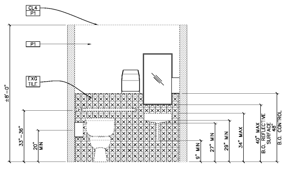
2 TOILET ROOM ELEVATION A5c SCALE 1/2" = 1'-0"
