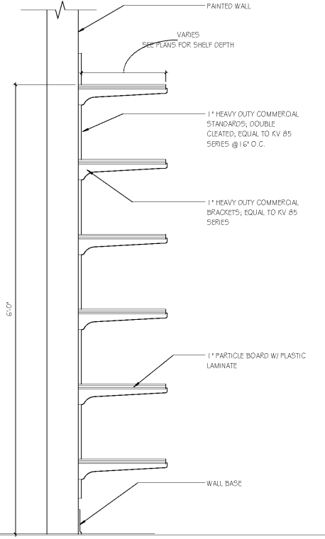
A7 TYPICAL STORAGE CLOSET SHELVING SCALE: 1/2" = 1'-0"
