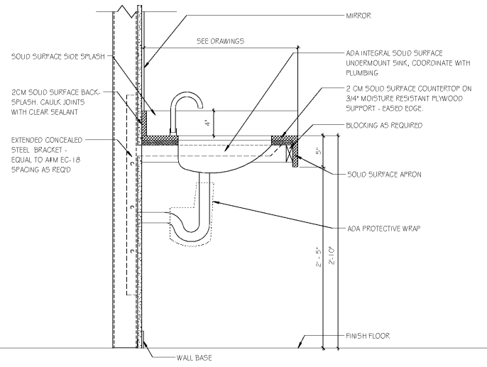
A9 SOLID SURFACE SINK COUNTER -ADA SCALE: 1/2" = 1'-0"
