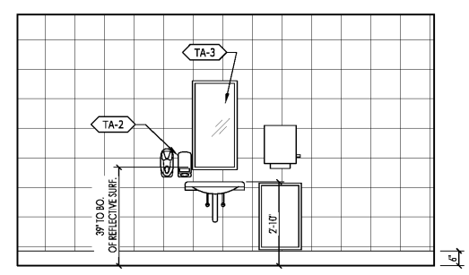
05 INT. ELEV @ WOMEN'S A7.1 SCALE: 3/8"= 1'-0"
