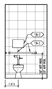
04 INT. ELEV @ MEN'S A7.1 SCALE: 3/8"= 1'-0"
