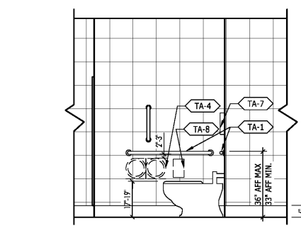
07 INT. ELEV @ WOMEN'S A7.1 SCALE: 3/8"= 1'-0"
