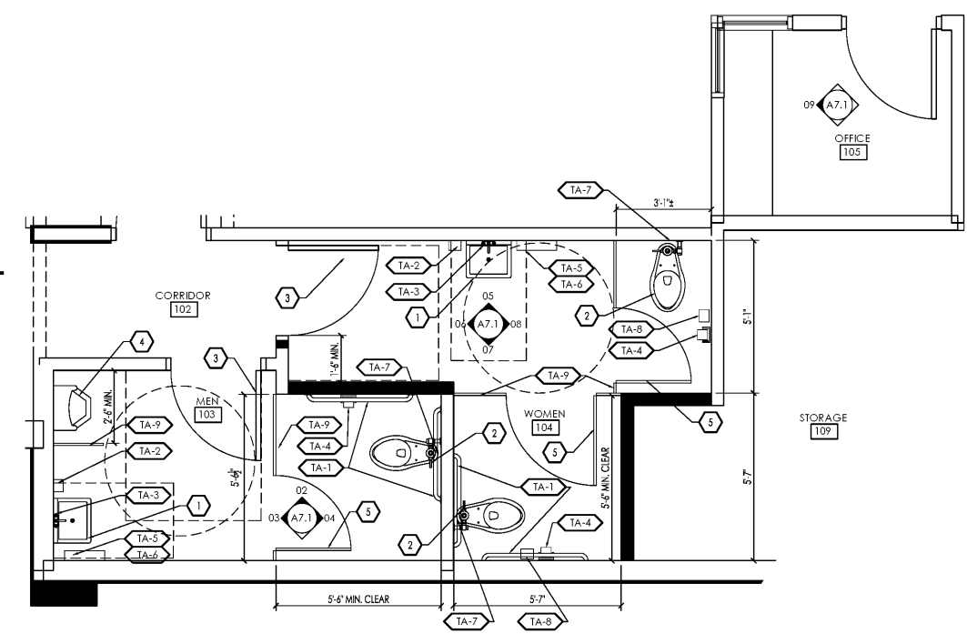
01 ENLARGED RESTROOM PLAN A7.1 SCALE: 3/8"= 1'-0"
