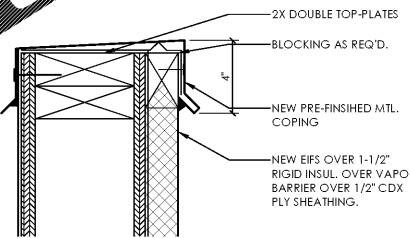
03 DETAIL @ NEW PARAPET CAP A5.3 SCALE: 3" = 1'-0"
