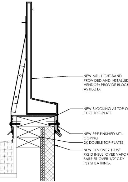
02 DETAIL @ NEW LIGHT BAND A5.3 SCALE: 3" = 1'-0"
