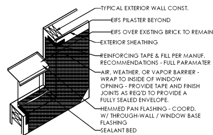
05 TYP. FLASHING DETAIL A5.3 SCALE: 3/4" = 1'-0"
