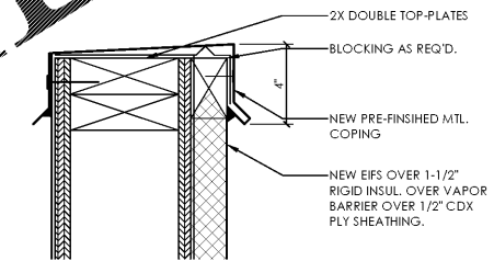
03 DETAIL @ NEW PARAPET CAP A5.3 SCALE: 3" = 1'-0"
