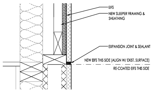
01 DETAIL @ EIFS / MASONRY JOINT A5.3 SCALE: 3" = 1'-0"
