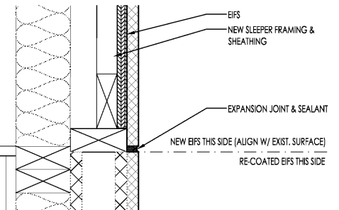
01 DETAIL @ EIFS / MASONRY JOINT A5.3 SCALE: 3" = 1'-0"
