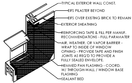
05 TYP. FLASHING DETAIL A5.3 SCALE: 3/4" = 1'-0"
