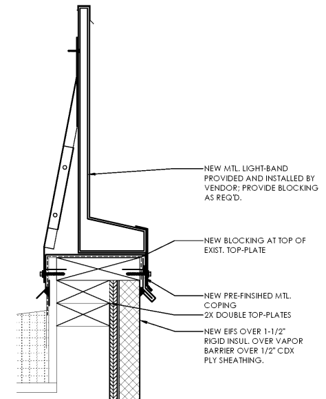
02 DETAIL @ NEW LIGHT BAND A5.3 SCALE: 3" = 1'-0"
