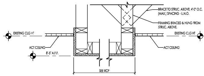
02 SOFFIT DETAIL @ SERVING COUNTER A3.1 SCALE: 1-1/2" = 1'-0"
