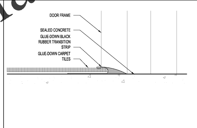
3 CONCRETE TO CARPET TRANSITION SCALE 6\"/>
