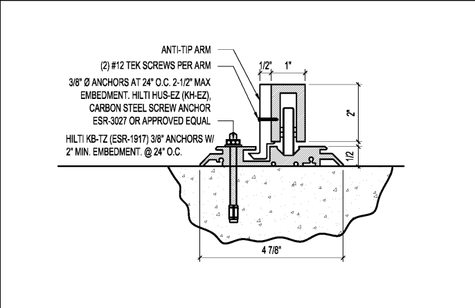
1 STOCK UNIT TRACK DETAIL SCALE 6\"/>
