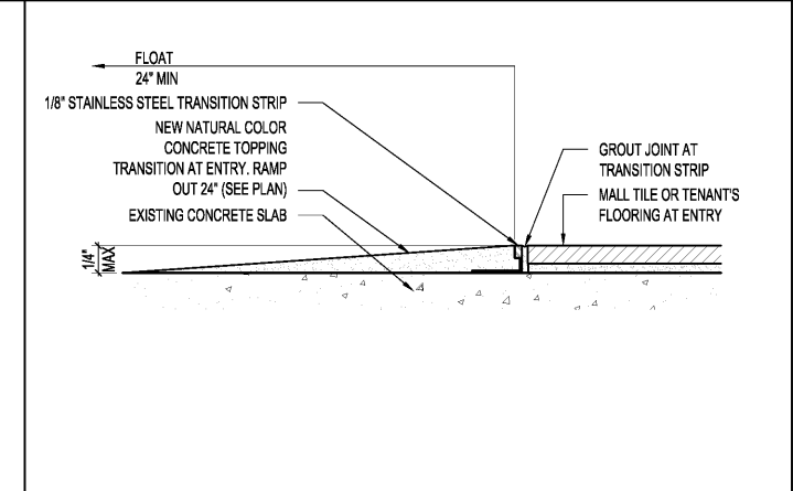
2 MALL TILE TO CONCRETE TRANSITION SCALE 6\"/>
