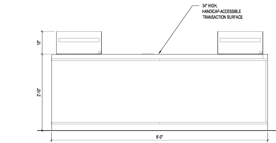
B FRONT CASHWRAP ELEVATION
