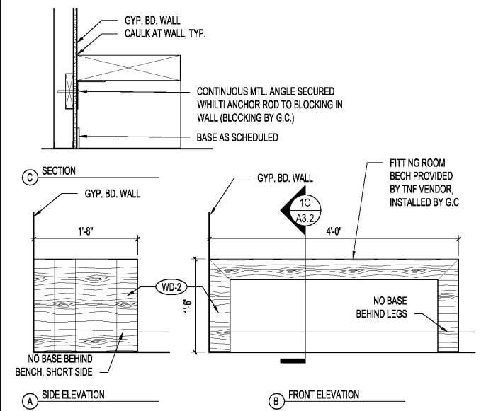
1 FITTING ROOM BENCH DETAIL
