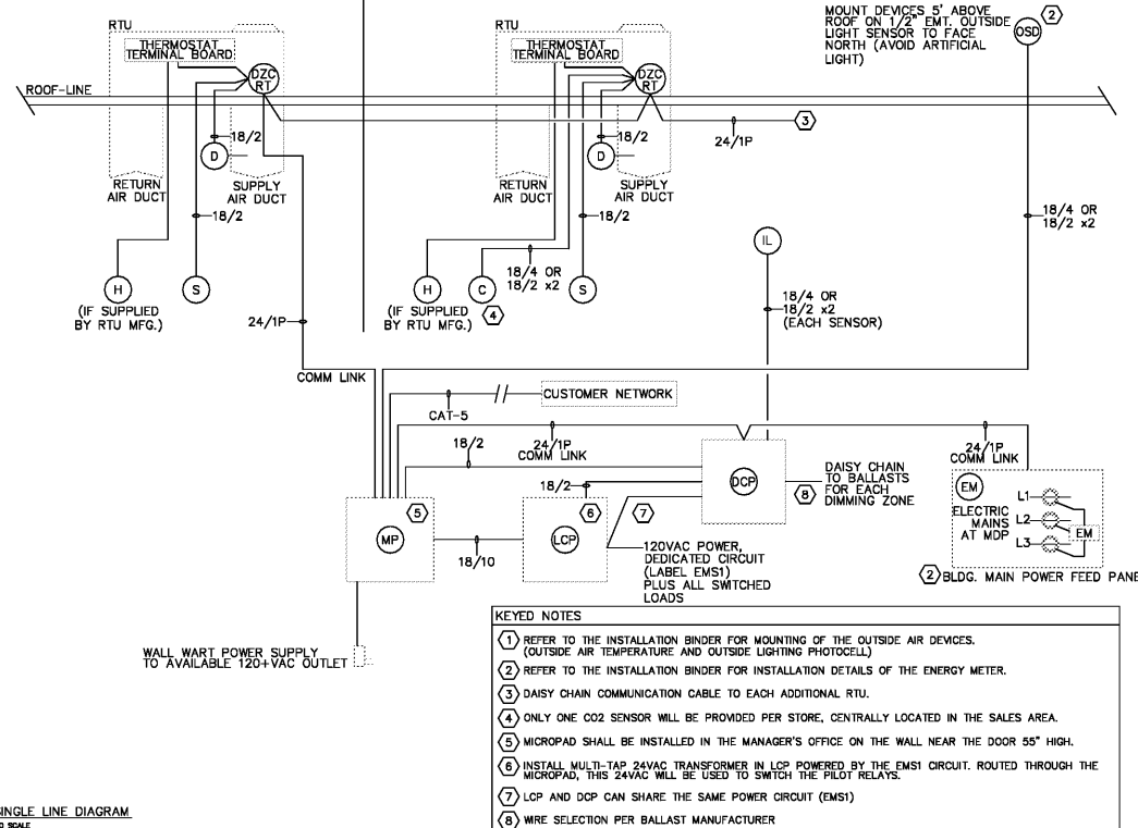
S SINGLE LINE DIAGRAM 1 NO SCALE
