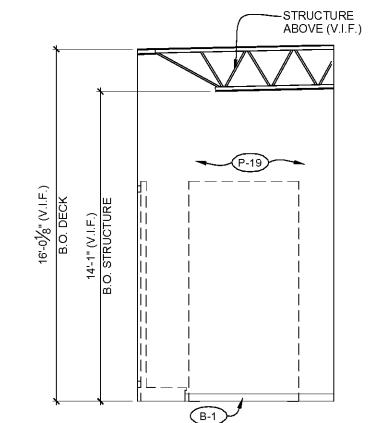
5 RECEIVING/STAGING ELEVATION A803 1/4" = 1'-0"
