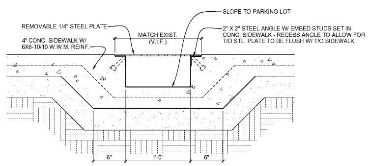
6 DRAINAGE TRENCH THRU SIDEWALK A803 1 1/2" = 1'-0"
