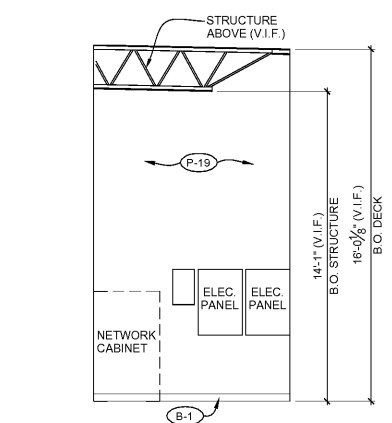
4 RECEIVING/STAGING ELEVATION A803 1/4" = 1'-0"
