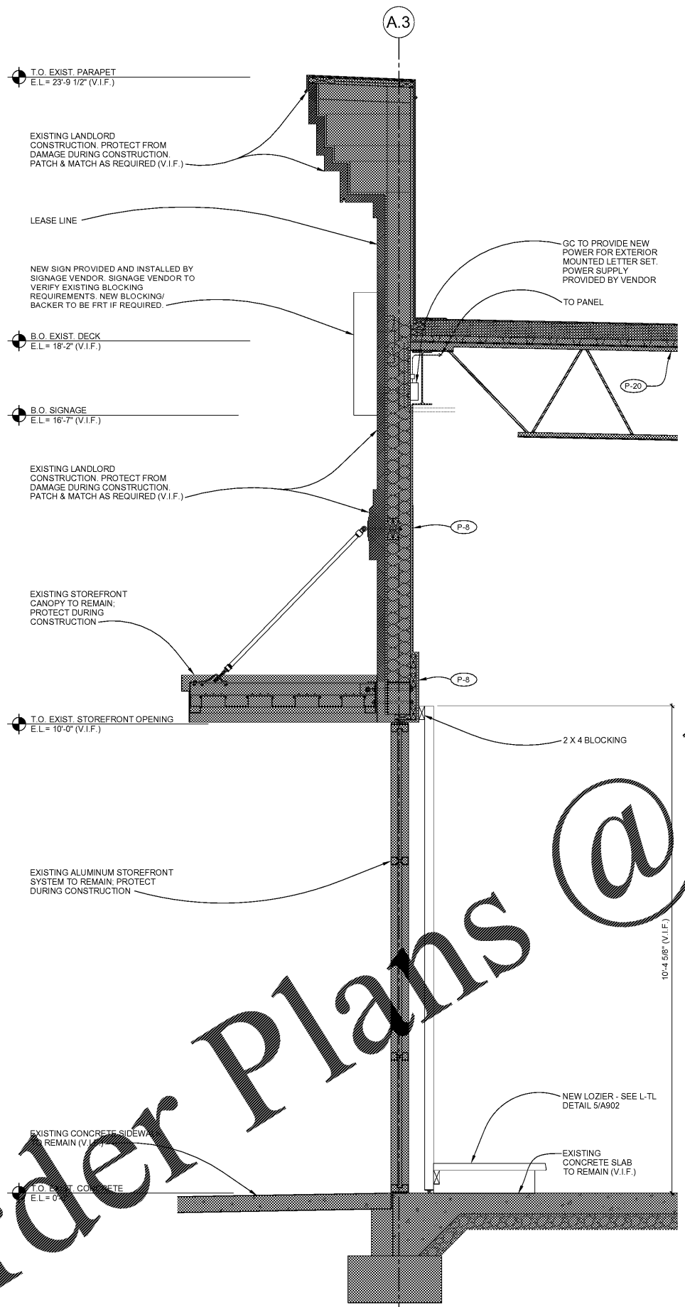
1 STOREFRONT SECTION 3/4" = 1'-0"
