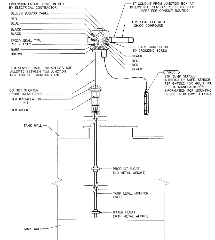
1 TANK LEVEL MONITOR (TLM) IN STP SUMP NTS
