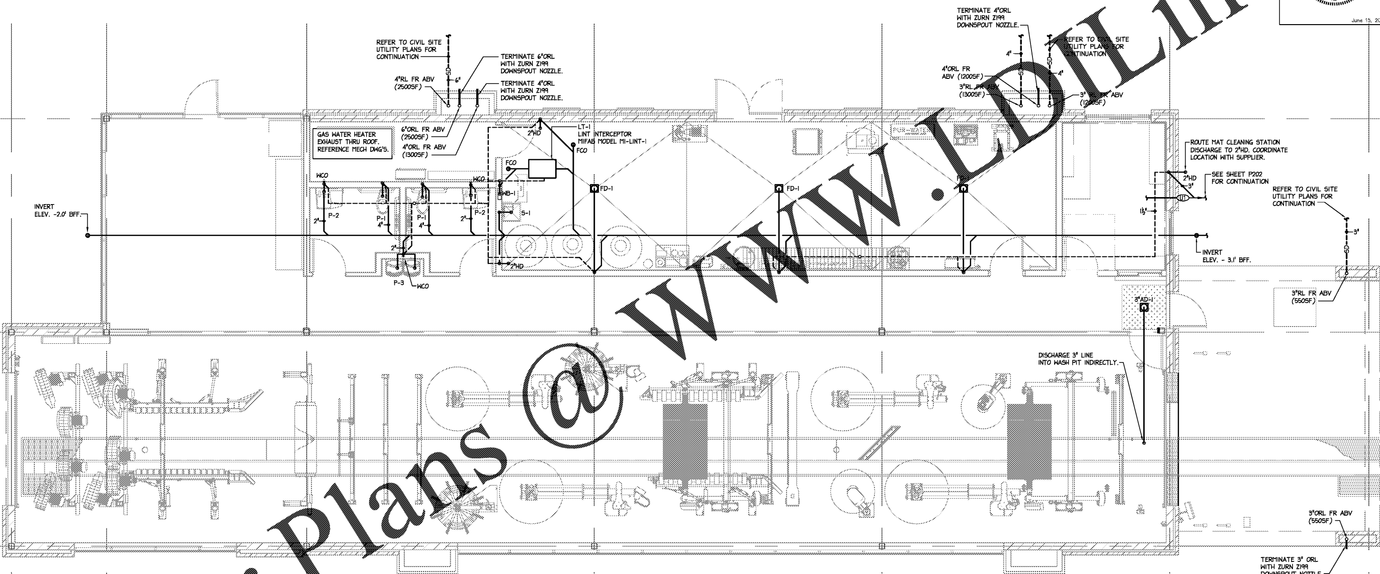
1 PLUMBING WASTE FLOOR PLAN 1/4" = 1'-0" NOTE: UNLESS OTHERWISE SPECIFIED, 1/4" PER FOOT SLOPE.
