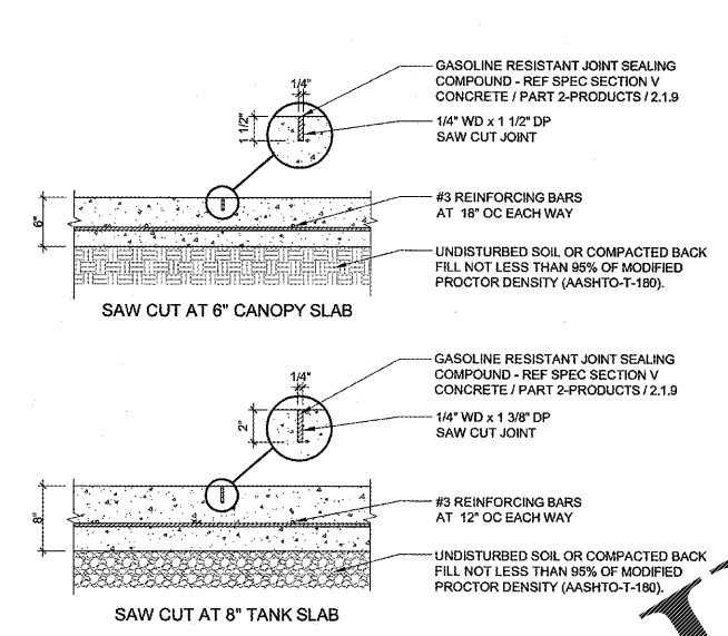
3 SAW CUT DETAILS
