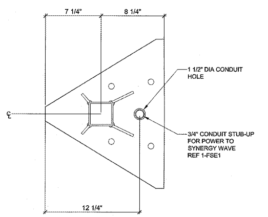
6 SYNERGY WAVE BASE DETAIL
