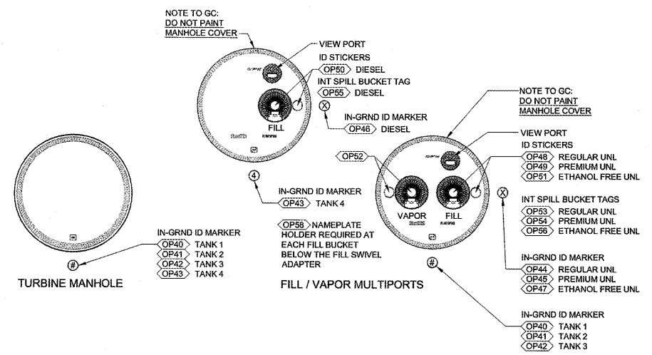
4 CONCRETE TAG AND MARKER DETAILS
