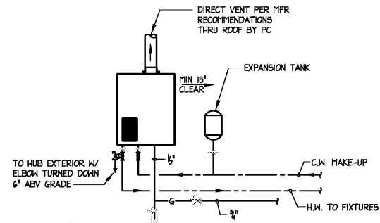
1 INSTANTANEOUS WATER HEATER DETAIL NO SCALE
