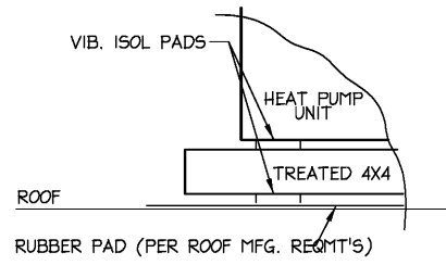
6 CONDENSING UNIT PAD DETAIL NO SCALE
