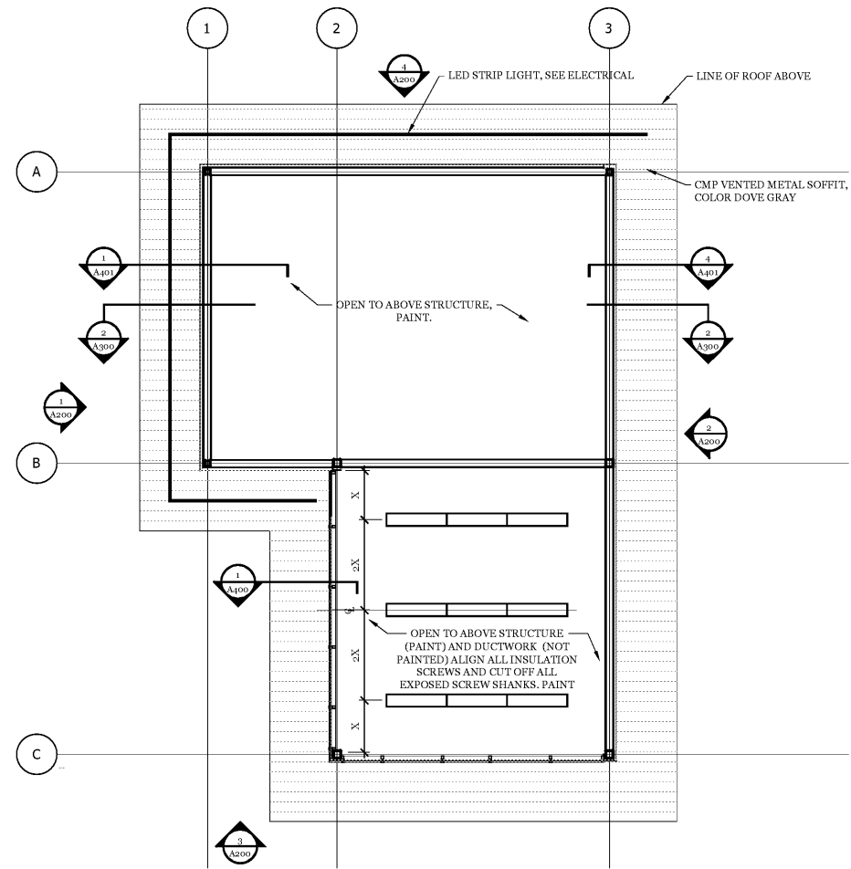
2 Tower Reflected Ceiling Plan 3/16" = 1'-0"
