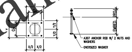
1 FOUNDATION PLAN SS03 SCALE: 3/8"=1'-0"
