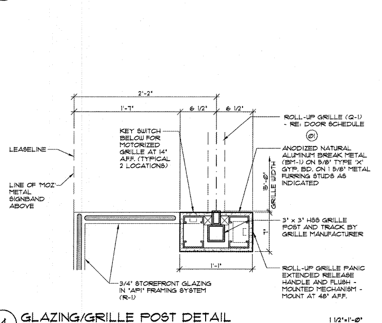
4 GLAZING/GRILLE POST DETAIL 1/2"x1'-0"
