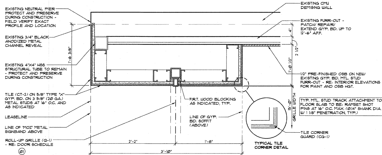
5 NEUTRAL PIER/GRILLE POST DETAIL 1/2"x1'-0"
