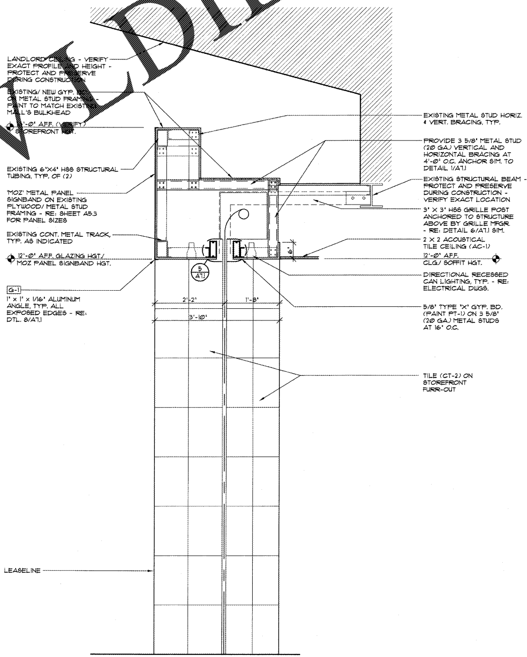
1 WALL SECTION AT GRILLE 3/4"x1'-0"
