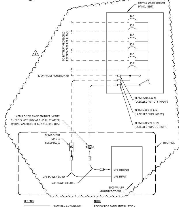
13 E300 BYPASS DISTRIBUTION PANEL WIRING DIAGRAM N.T.S.
