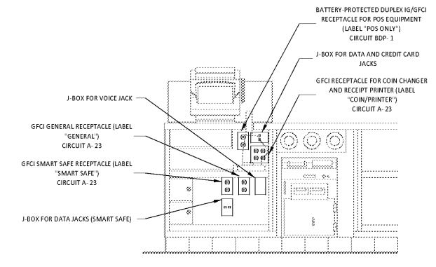
6 E300 POS COUNTER ELECTRICAL ELEVATION N.T.S.
