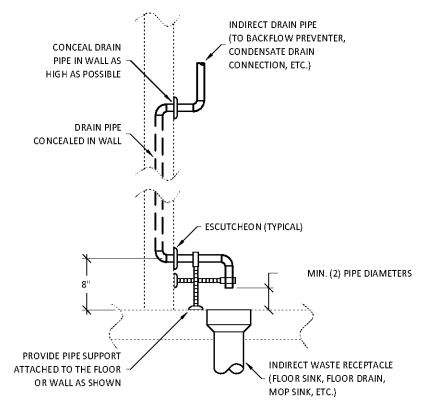
10 INDIRECT WASTE PIPING DETAIL P300 N.T.S.
