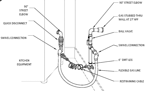
2 KITCHEN GAS EQUIPMENT DETAIL P300 N.T.S.
