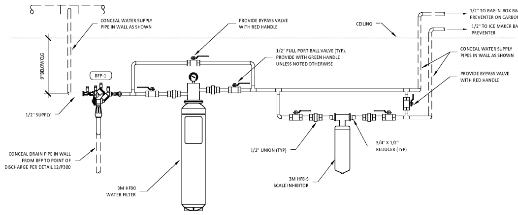
11 WATER FILTRATION DETAIL P300 N.T.S.
