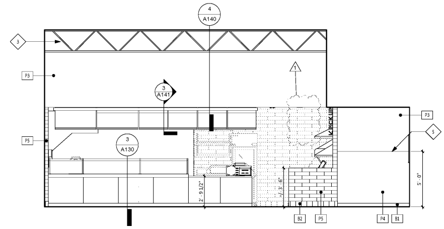
2 ORDERING ELEVATION 1/4" = 1'-0"
