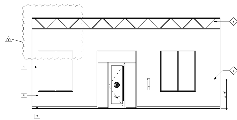
1 MAIN ENTRY ELEVATION 1/4" = 1'-0"
