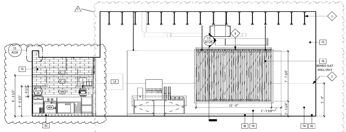
4 DINING ELEVATION 1/4" = 1'-0"
