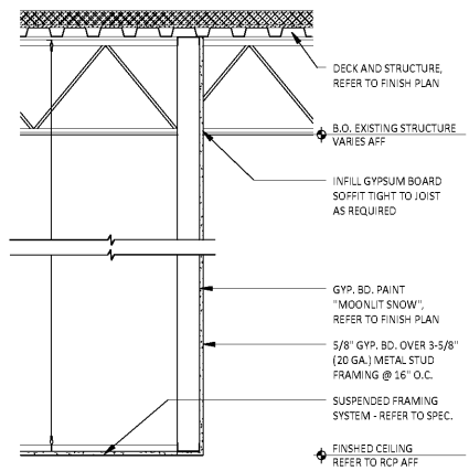
SECTION @ SOFFIT A140 3/4" = 1'-0"
