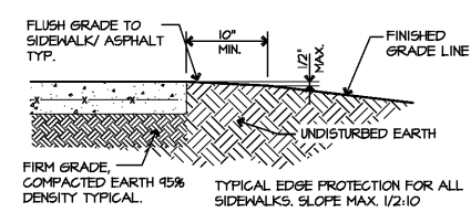
3 TYP. CONDITION SIDEWALK EDGE @ GRADE SCALE: 1" = 1'-0"
