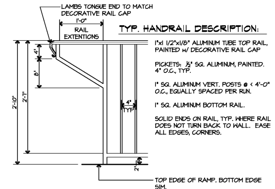
5 TYP. @ ALL RAMP HANDRAIL DETAIL SCALE: 1" = 1'-0"
