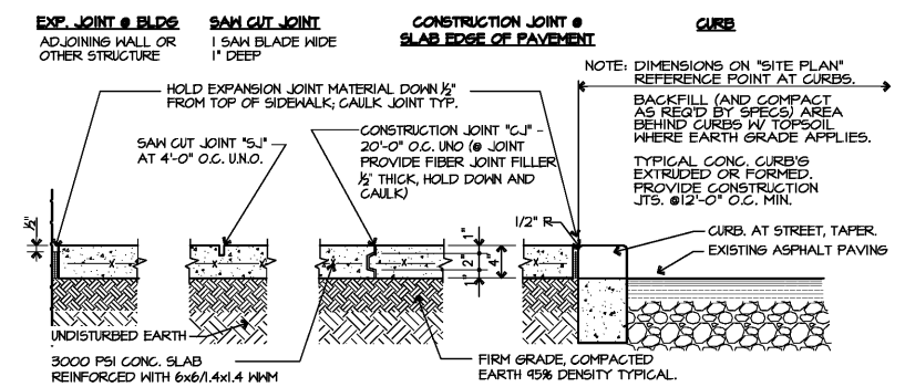
4 TYP. CONDITIONS @ SIDEWALK DETAILS SCALE: 1" = 1'-0"
