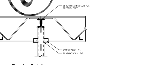
19 Framing Detail SCALE: 3/4" = 1'-0"
