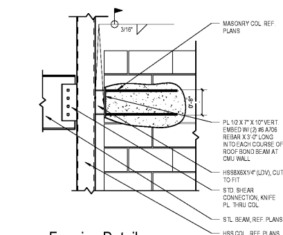
7 Framing Detail SCALE: 3/4" = 1'-0"
