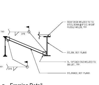
8 Framing Detail SCALE: 3/4" = 1'-0"
