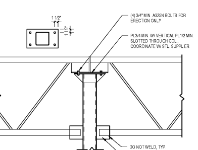
16 Framing Detail SCALE: 3/4" = 1'-0"
