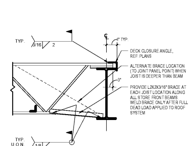
13 Framing Detail SCALE: 3/4" = 1'-0"
