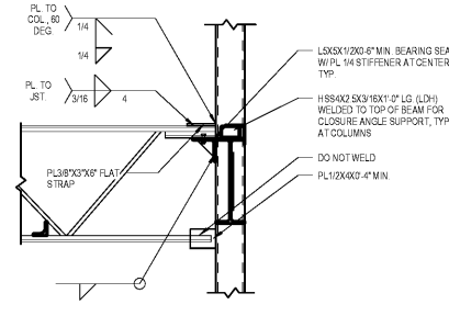
12 Framing Detail SCALE: 3/4" = 1'-0"
