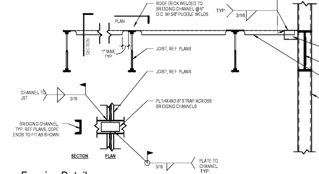
9 Framing Detail SCALE: 3/4" = 1'-0"
