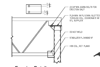
17 Framing Detail SCALE: 3/4" = 1'-0"
