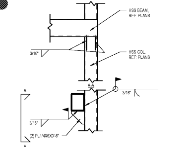
15 Framing Detail SCALE: 3/4" = 1'-0"
