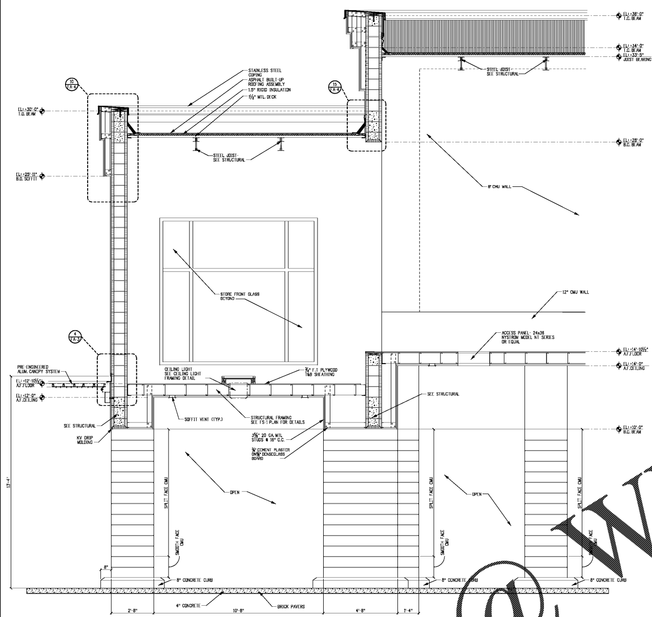
1 WALL SECTION @ TOWERS FA-3 SCALE: 1/2" = 1'-0"
