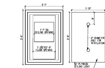
3 FRONT WALL SECTION FA-3 SCALE: 1/2" = 1'-0"
