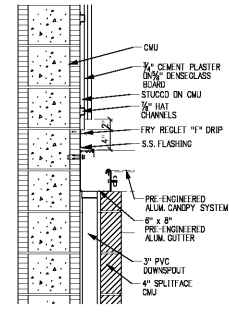
8 CANOPY CONNECTION DETAIL AT PILASTER FA-3 SCALE: 1" = 1'-0"
