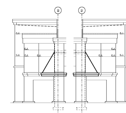
6 PARTIAL SIDE ELEVATION FA-2 SCALE: 1/2"=1'-0"
