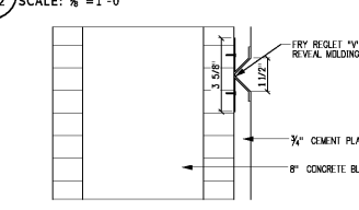
5 REVEAL DETAIL FA-2 SCALE: 1/2"=1'-0"
