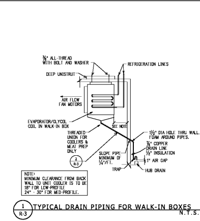
1 TYPICAL DRAIN PIPING FOR WALK-IN BOXES N.T.S.
