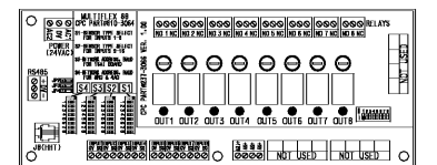
3 TYP. MULTIFLEX 88 I/O BOARD AT A/C UNIT
