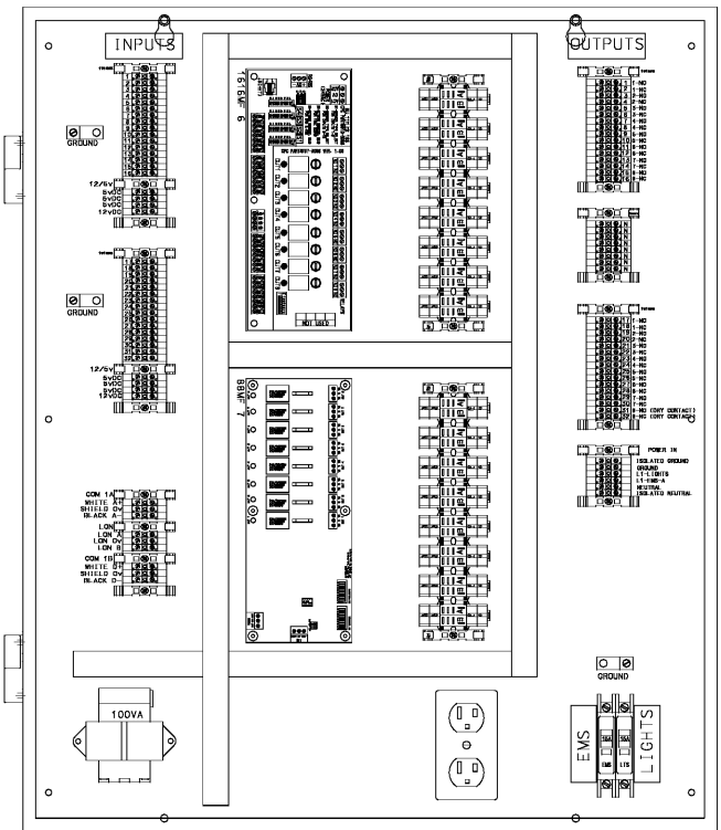
EMS A INTERIOR ELEVATION
