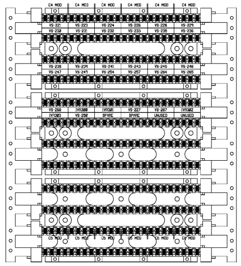
TYP. VOICE STATION TERMINAL BLOCK N/A
