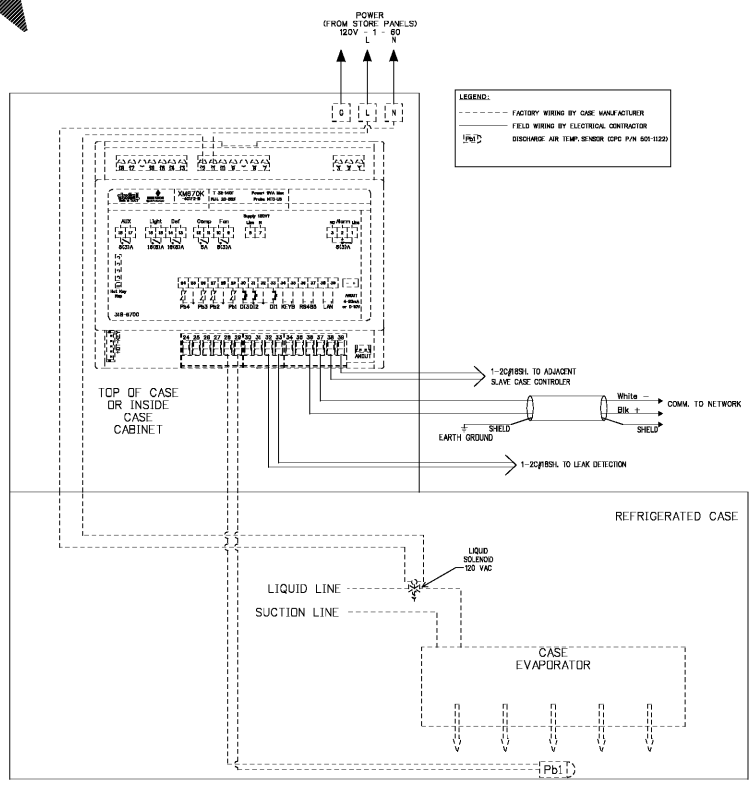
4 CASE WIRING DIAGRAM - MED. TEMP. E-46 (TIMED OFF DEFOST, REFRIGERATED CASE) N.T.S.
