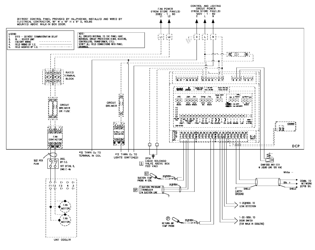
1 DCP WIRING DIAGRAM E-44 (TIMED OFF DEFOST, WALK-IN W/ONE COIL) N.T.S.
