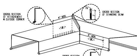
5 CORNER COPING SEAM DETAIL RD-2 SCALE: NONE
