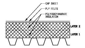
4 ROOF R-VALUE DETAIL RD-2 SCALE: 3"=1'-0"
