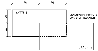
4 ROOF R-VALUE DETAIL RD-2 SCALE: 3"=1'-0"
