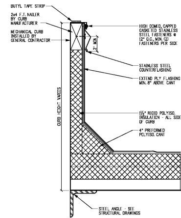
2 EQUIPMENT CURB DETAIL RD-2 SCALE: 3"=1'-0"
