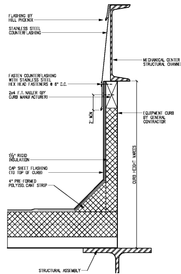
1 MECHANICAL CENTER CURB DETAIL RD-2 SCALE: 3"=1'-0"
