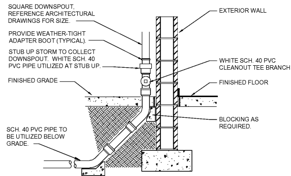
1 DOWNSPOUT SHOE INSTALLATION P5 SCALE: N.T.S.
