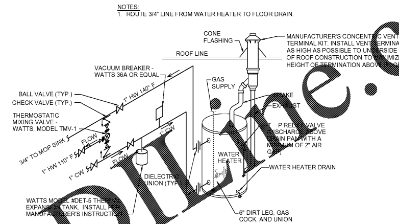
3 GAS FIRED WATER HEATER SECTION P5 SCALE: N.T.S.
