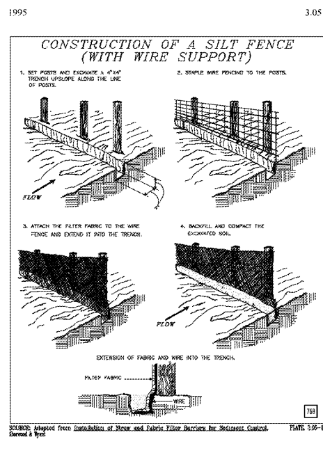
SILT FENCE
