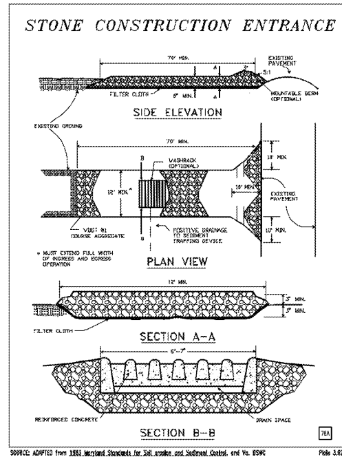
STONE CONST. ENTRANCE
