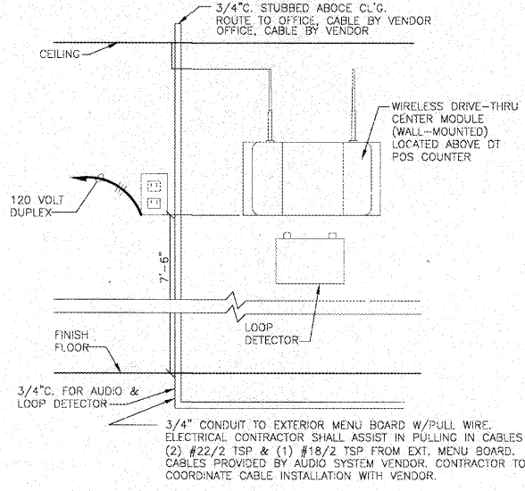
DRIVE THRU AUDIO SYSTEM DETAIL
