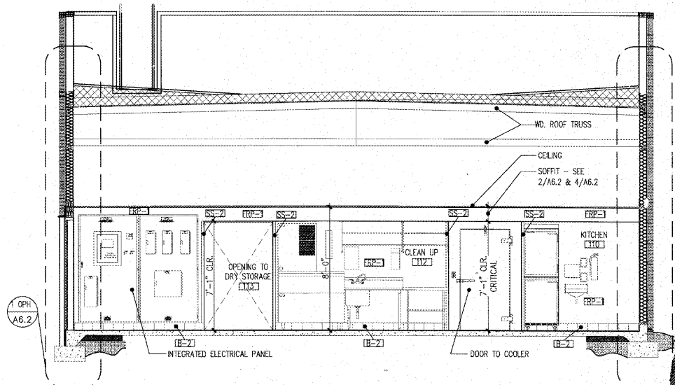
INTERIOR ELEVATION / BLDG. SECTION
