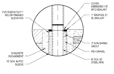
11 ENLARGED BOLLARD DETAIL 1" x 1'-0"
