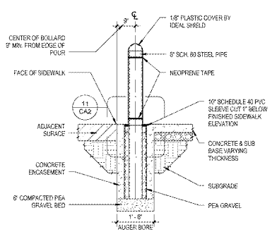
5 BOLLARD DETAIL 1/2" x 1'-0"
