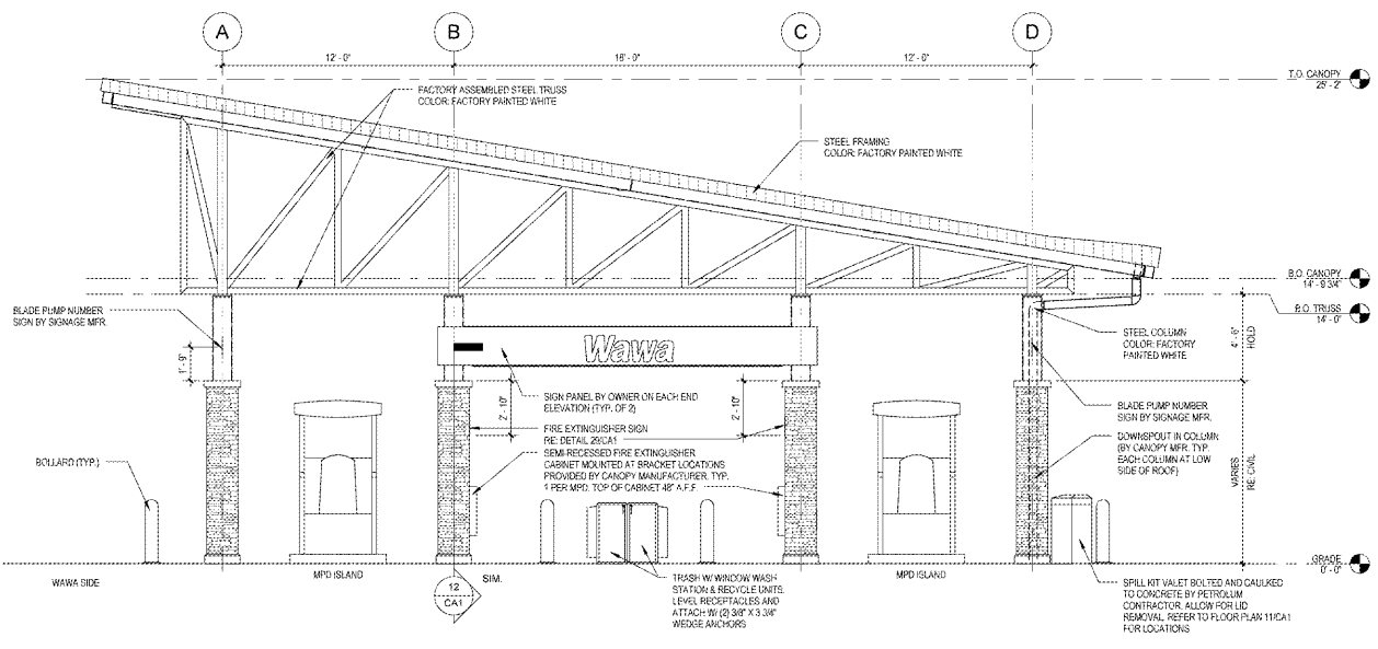
27 CANOPY ELEVATION 14'-0" x 12'-0"
