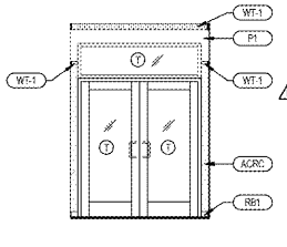
8 REAR VESTIBULE ELEVATION A8.2 1/4" x 1/4"
