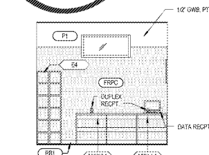
18 ASSOCIATE'S ROOM ELEV. A8.2 1/4" x 1/4"
