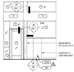
4 FRONT VESTIBULE ELEVATION A8.2 1/4" x 1/4"
