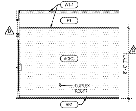
9 REAR VESTIBULE ELEVATION A8.2 1/4" x 1/4"
