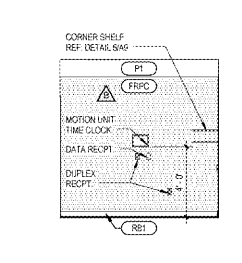
10 OFFICE ELEVATION A8.2 1/4" x 1/4"
