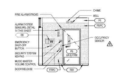
11 OFFICE ELEVATION A8.2 1/4" x 1/4"
