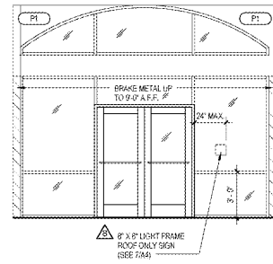
3 FRONT VESTIBULE ELEVATION A8.2 1/4" x 1/4"
