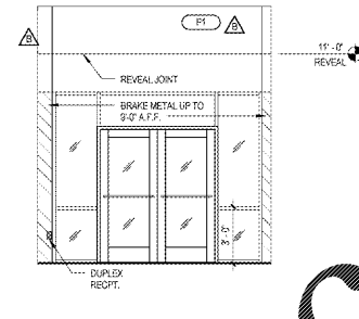
1 FRONT VESTIBULE ELEVATION A8.2 1/4" x 1/4"
