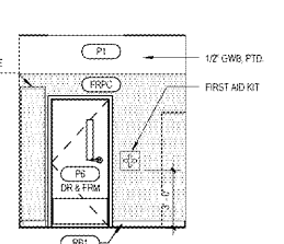
17 ASSOCIATE'S ROOM ELEV. A8.2 1/4" x 1/4"
