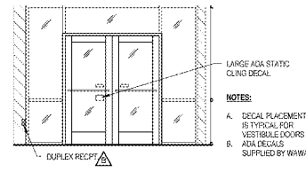
5 ADA DECAL DTL @ VESTIBULE DOOR A8.2 1/4" x 1/4"
