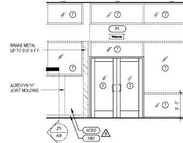
2 FRONT VESTIBULE ELEVATION A8.2 1/4" x 1/4"
