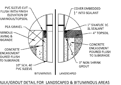
CAULK/GROUT DETAIL FOR LANDSCAPED & BITUMINOUS AREAS
