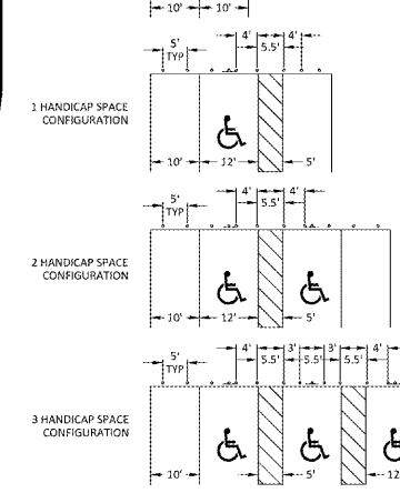
BOLLARD SPACING/DIMENSION DETAIL NTS
