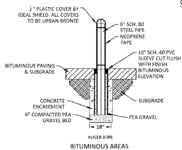
BOLLARD DETAIL NTS
