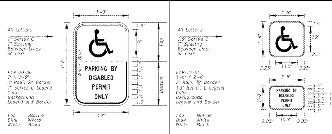
SPECIAL SIGN DETAILS INDEX NO. 17355 SHEET NO. 2 of 11
