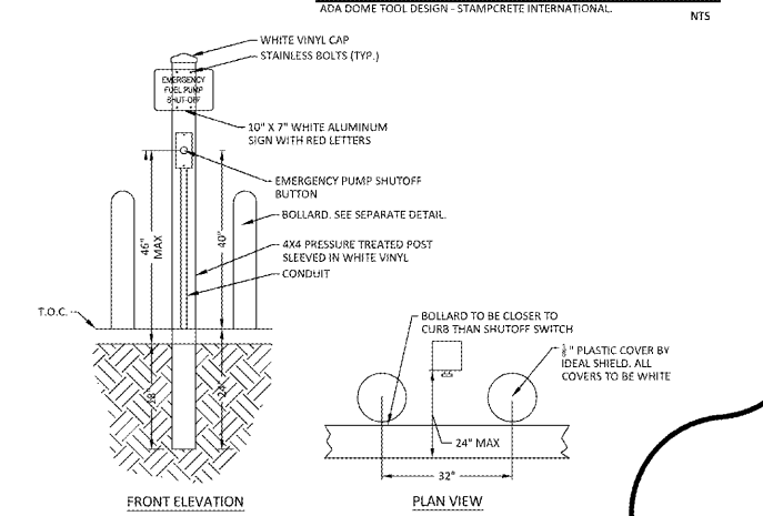
EMERGENCY PUMP SHUTOFF DETAIL NTS
