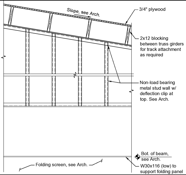
1 - Section
