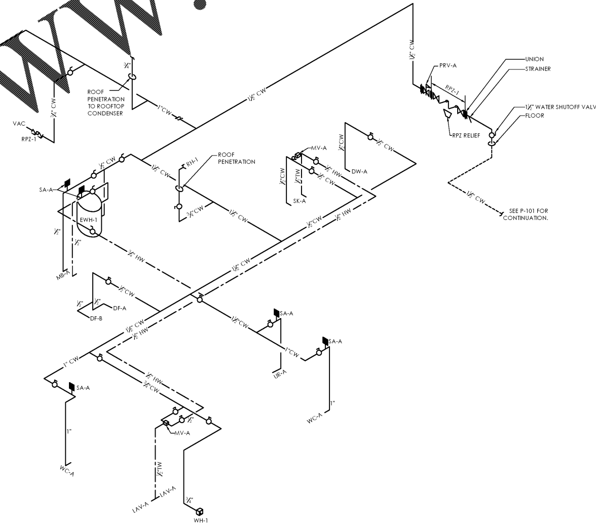
B1 Domestic Water Isometric Diagram NO SCALE
