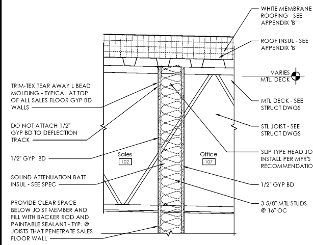
D3 Interior Section Detail - Interior Wall Head at Sales
