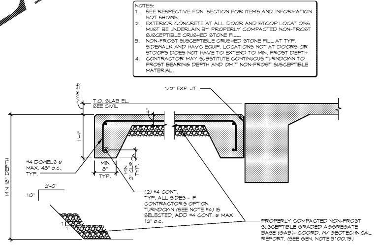
7 TYP. SIDEWALK & HVAC SLAB AT CONT. FTG SECTION 3/4" x 1'-0"
