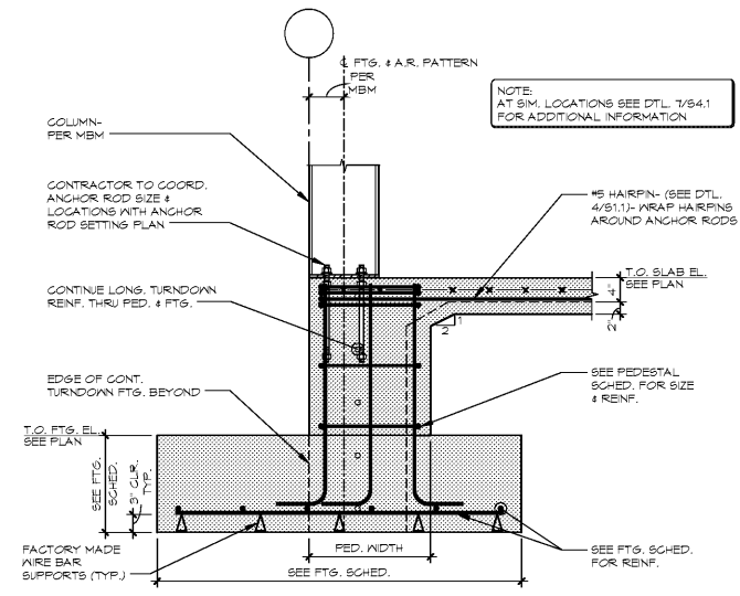
3 SECTION 3/4" x 1'-0"
