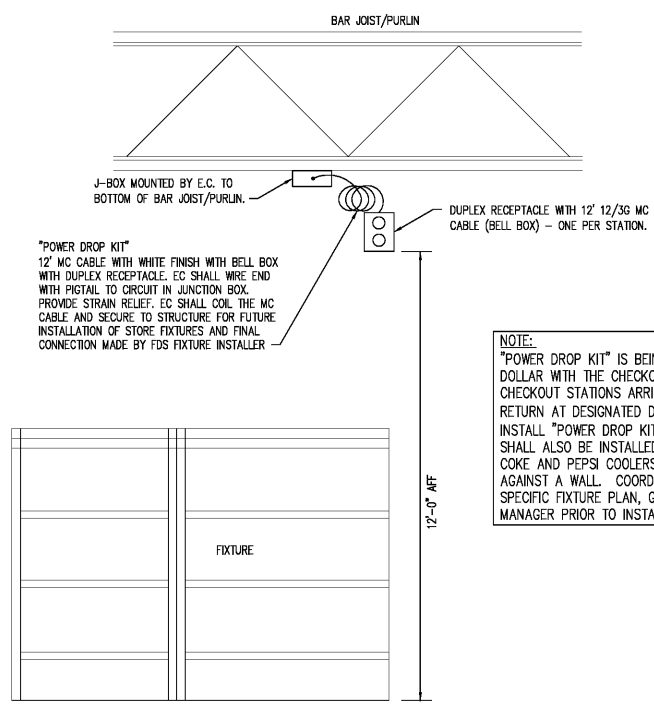
1 "POWER DROP KIT" INSTALLATION DETAIL N.T.S.
