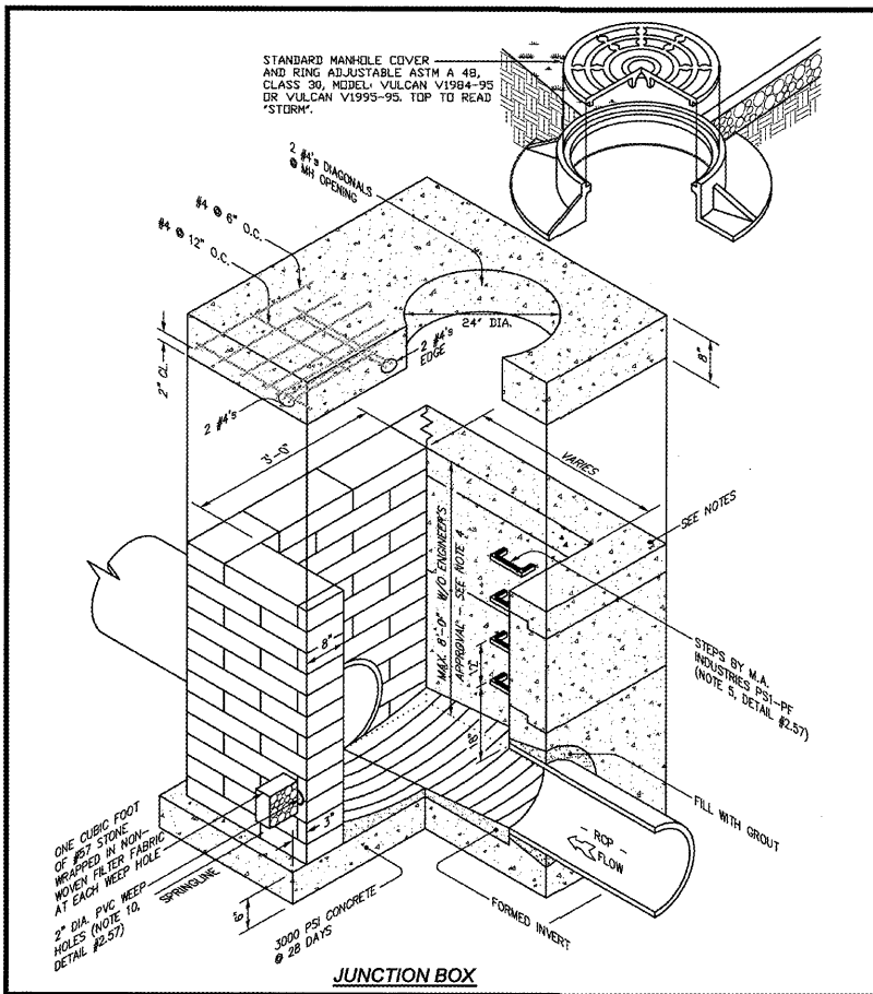
JUNCTION BOX
